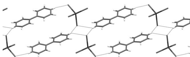
Figure 3. Crystal structure of [4,4'-H 2 bipy][FeCl 4 ] ( 7 ).
